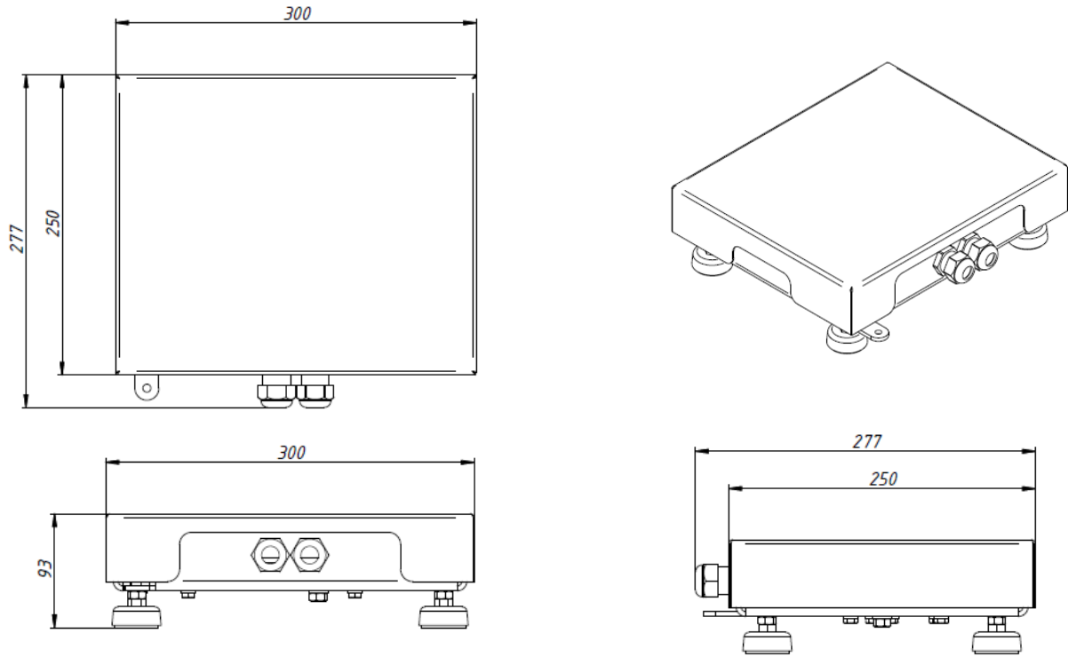
Dimensional drawing of indicator
